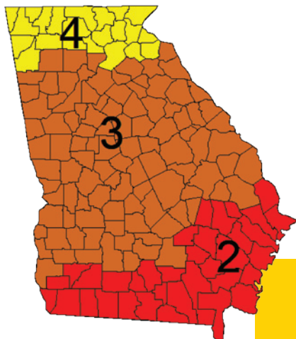
Figure 1. Georgia Climate Zones
