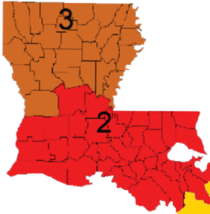
Figure 1. Louisiana Climate Zones
