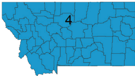
Figure 1. Montana Climate Zone
