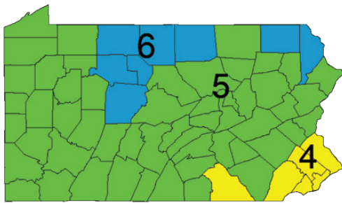
Figure 1. Pennsylvania Climate Zones
