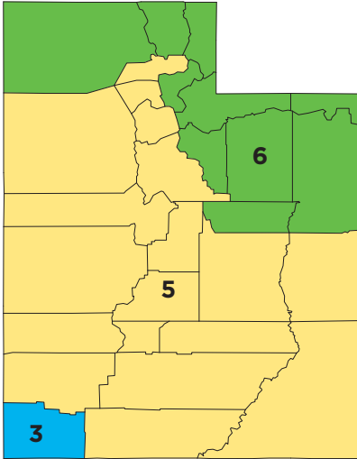
Figure 1. Utah Climate Zones
